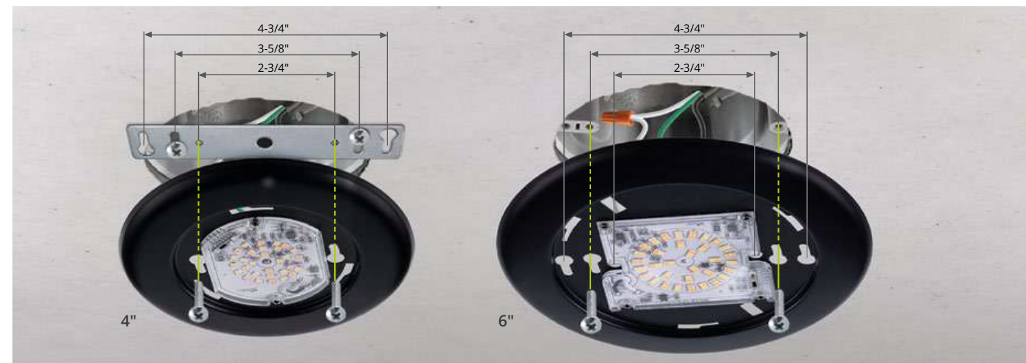
2.75", 3.5" AND 4" MOUNTING HOLES
