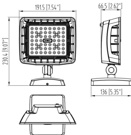
GRD32-PC-4K-BZ
