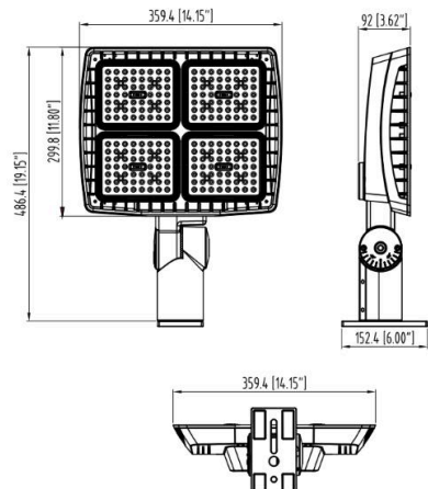
GRD150-PC-4K-BZ
